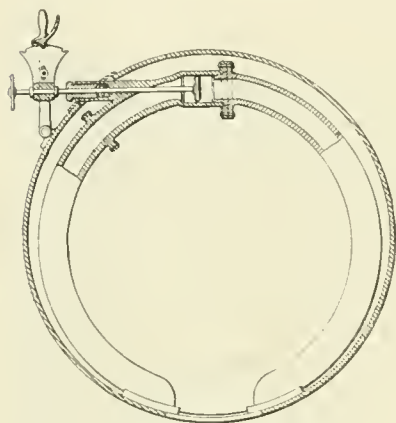
STOP VALVE IN LOCOMOTIVE BRANCH PIPES.
